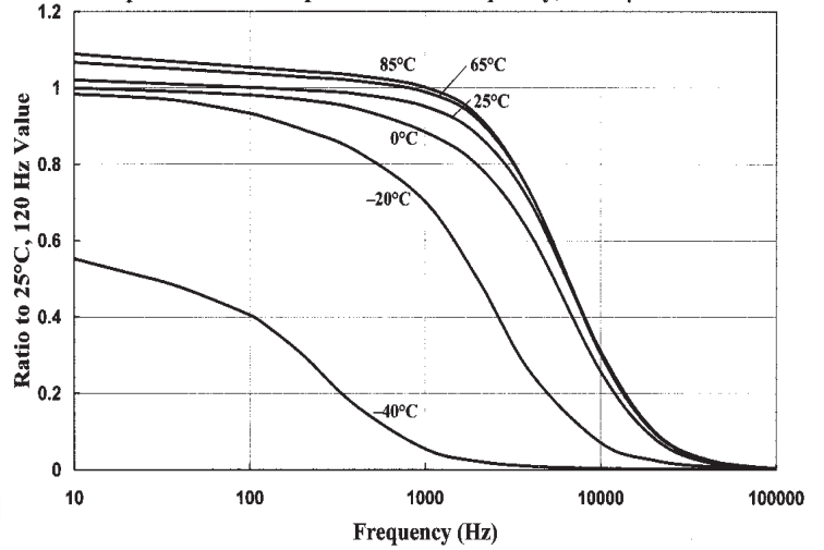
Capacitance vs Temperature and Frequency, 7900 \mu\text{F} 400 V
