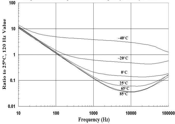
Impedance vs Temperature and Frequency, 4800 \mu\text{F} 200 V
