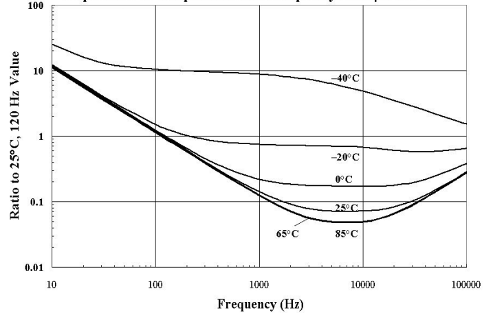
Impedance vs Temperature and Frequency 7900 \mu\text{F} 400 V
